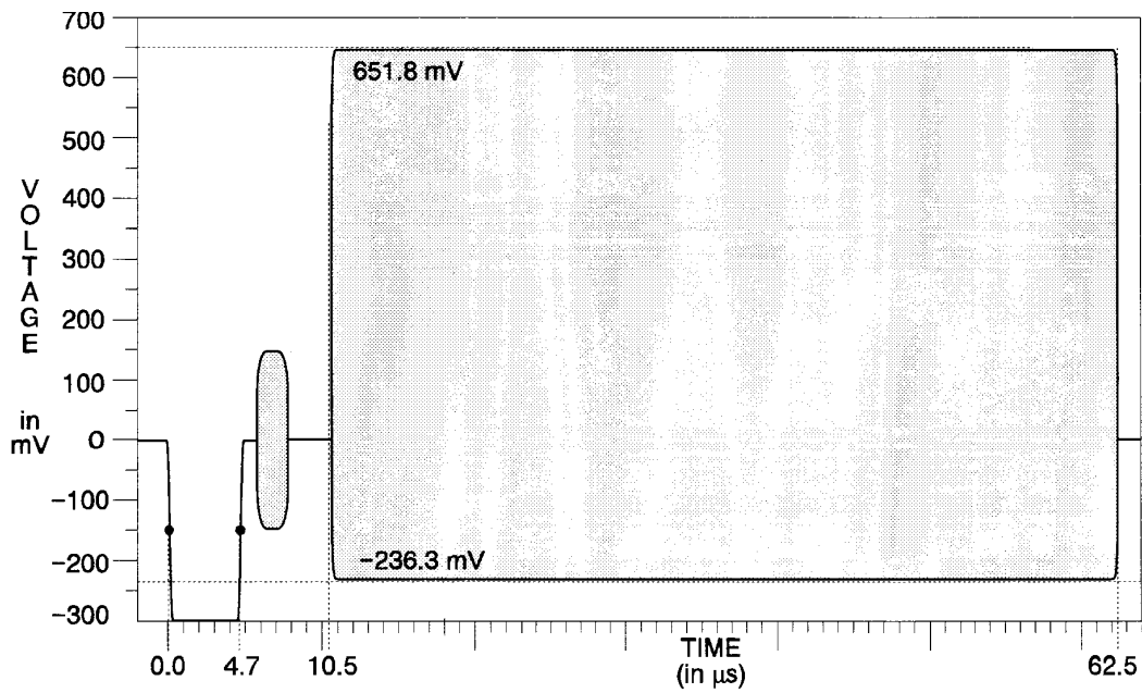
Figure 2-4: 100% red
