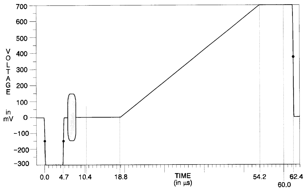
Figure 2-9: Ramp
