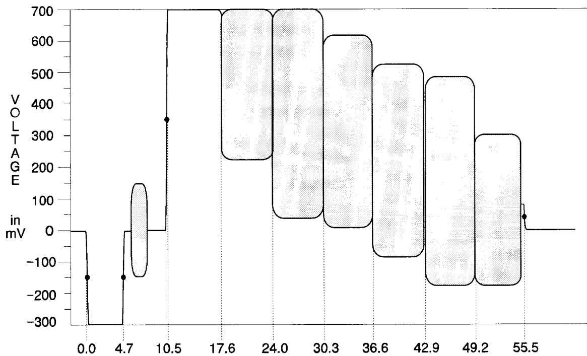
Figure 2-1: 75% color bars
