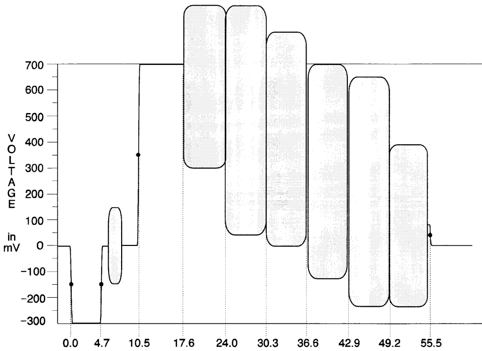
Figure 2-3: 100% color bars
