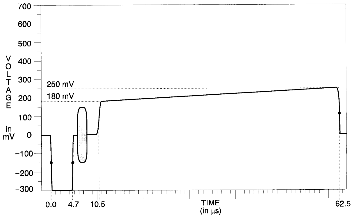
Figure 2-21: Shallow ramp
