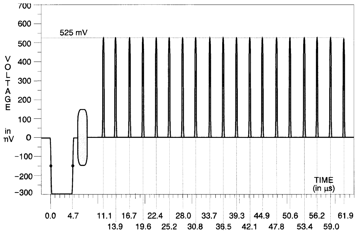
Figure 2-7: Convergence (vertical)
