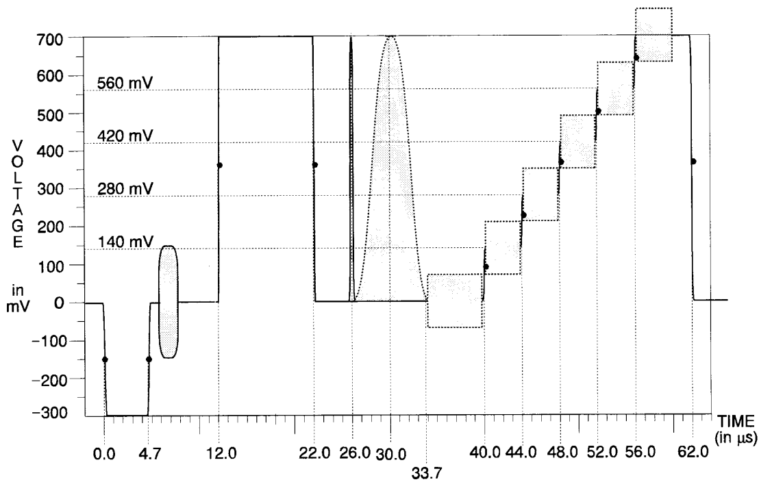
Figure 2-17: UK ITS 1
