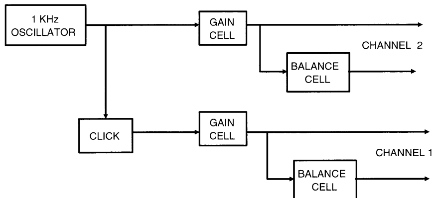
Figure 3-7: The Audio circuit <7>
