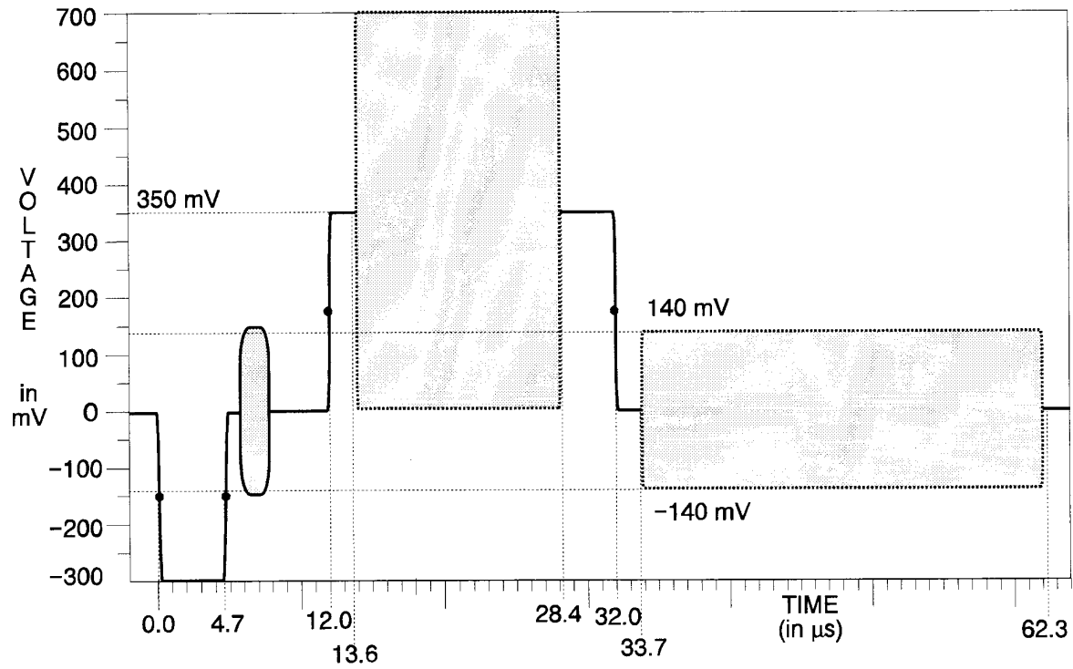
Figure 2-18: UK ITS 2
