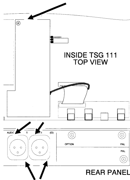
Figure 6-1: Remove these 5 Pozidriv screws to remove the Audio board from the instrument
